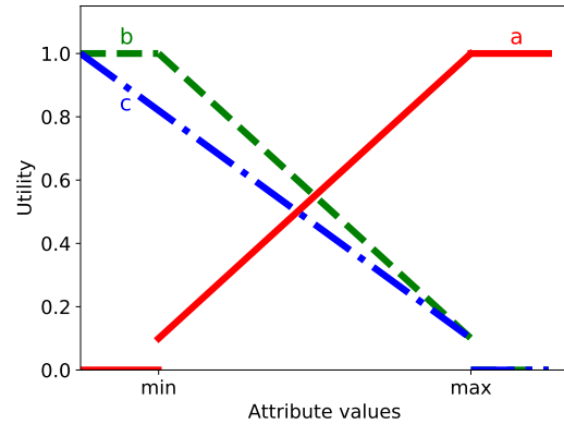
Figure 1: Utility functions.
