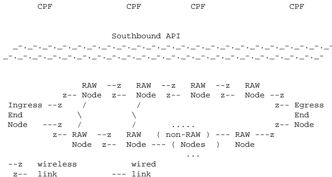
Figure 7: RAW Nodes
