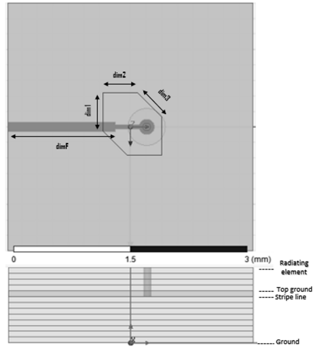
Fig. 1 – Antenna geometry
