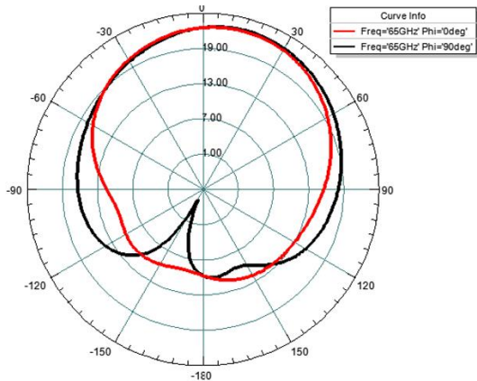
Fig. 8 – Polar radiation pattern for E plan and H plan
